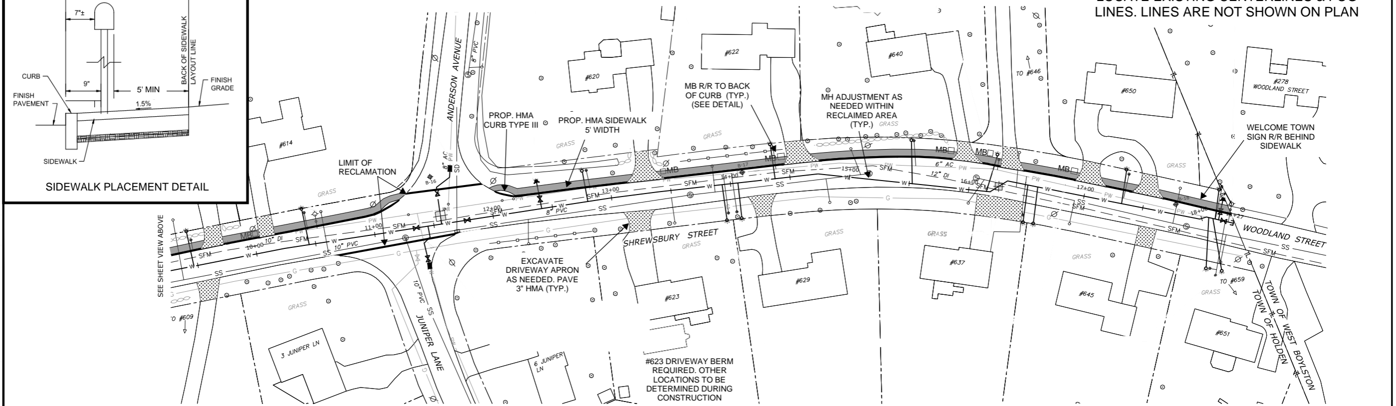
FIGURE 2 - SHREWSBURY STREET RECLAMATION & SIDEWALK PLAN JUNE 2023 - REV 1
